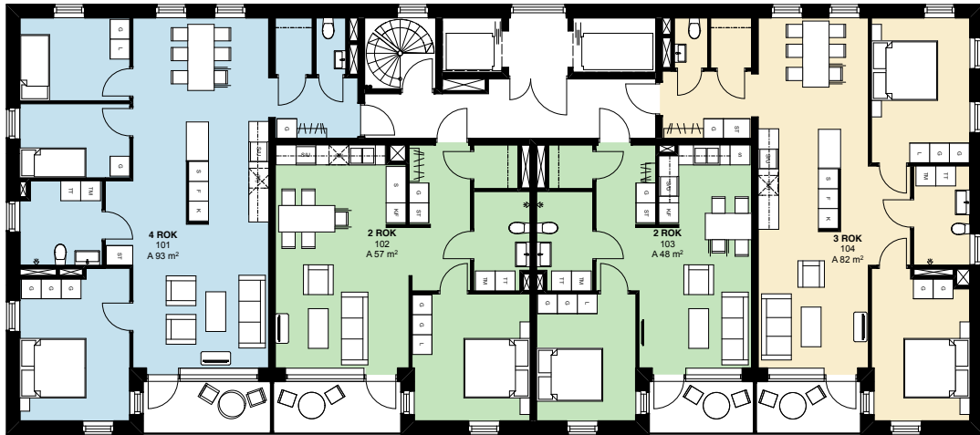
PLAN 10
