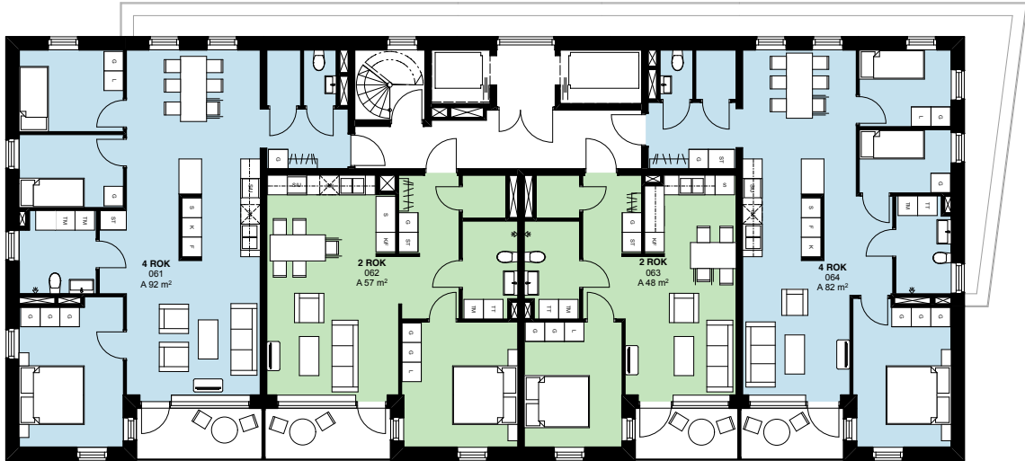
PLAN 6
