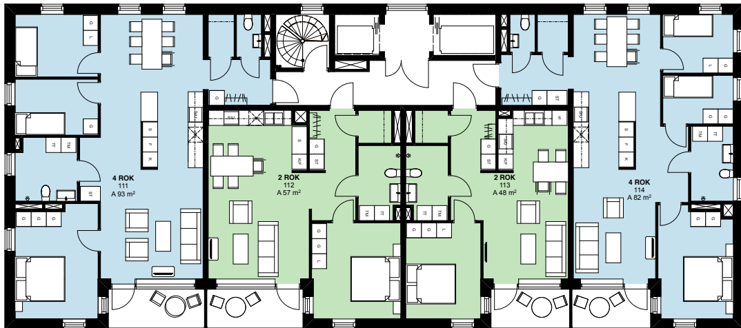
PLAN 11
