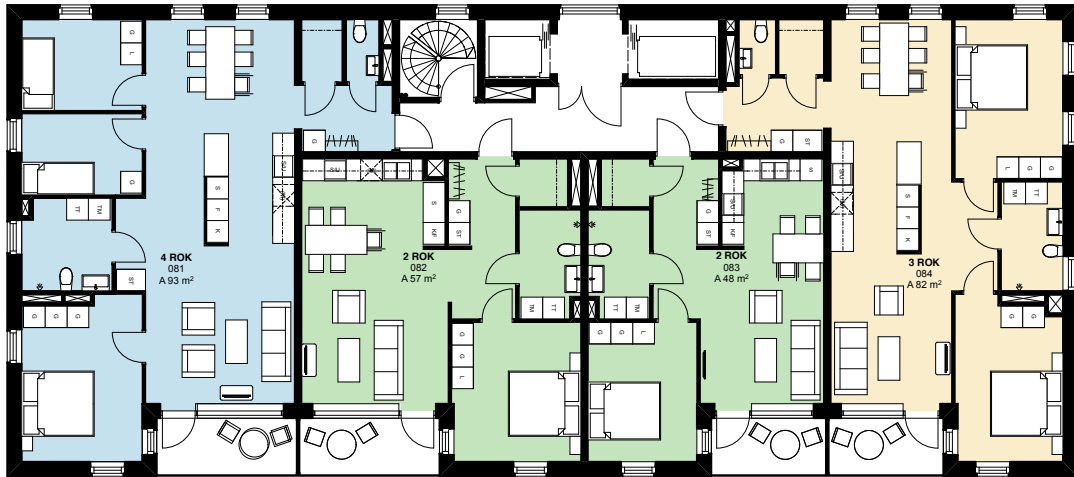
PLAN 8
