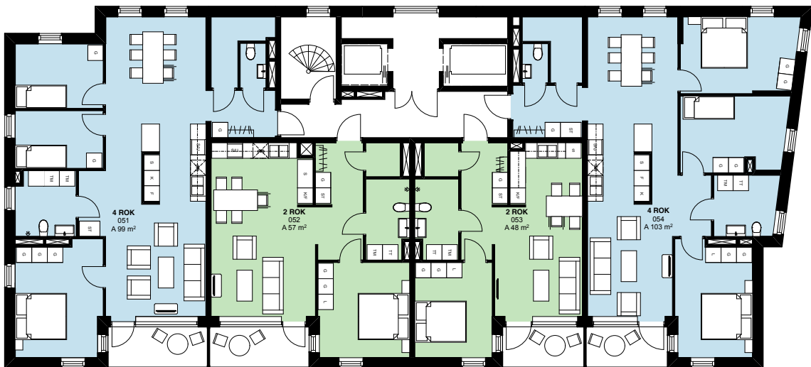
PLAN 5
